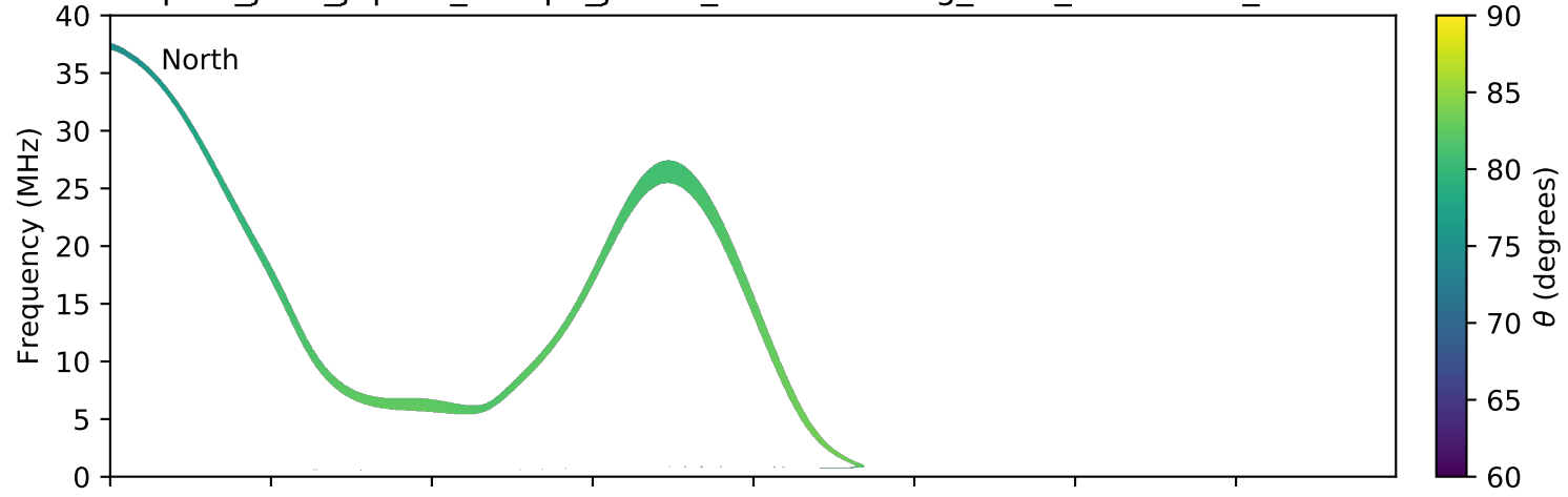
expres_juno_jupiter_europa_jrm09_lossc-wid1deg_3kev_20180221_v01.cdf
