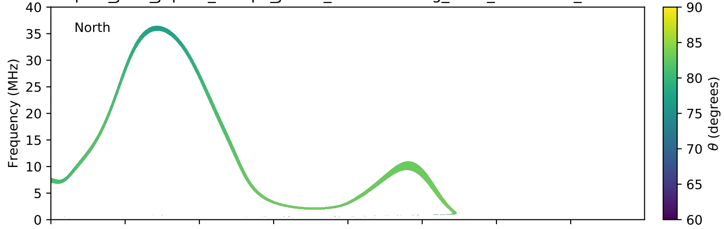
expres_juno_jupiter_europa_jrm09_lossc-wid1deg_3kev_20180220_v01.cdf
