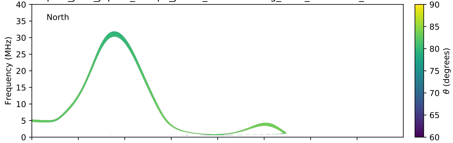
expres_juno_jupiter_europa_jrm09_lossc-wid1deg_3kev_20180215_v01.cdf
