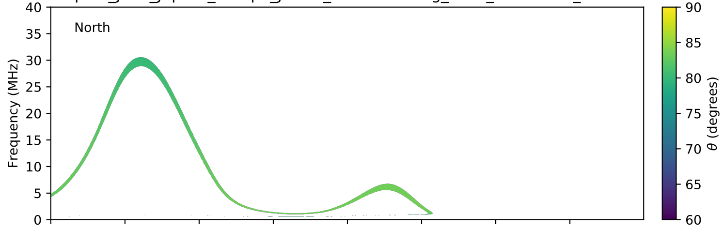
expres_juno_jupiter_europa_jrm09_lossc-wid1deg_3kev_20180213_v01.cdf
