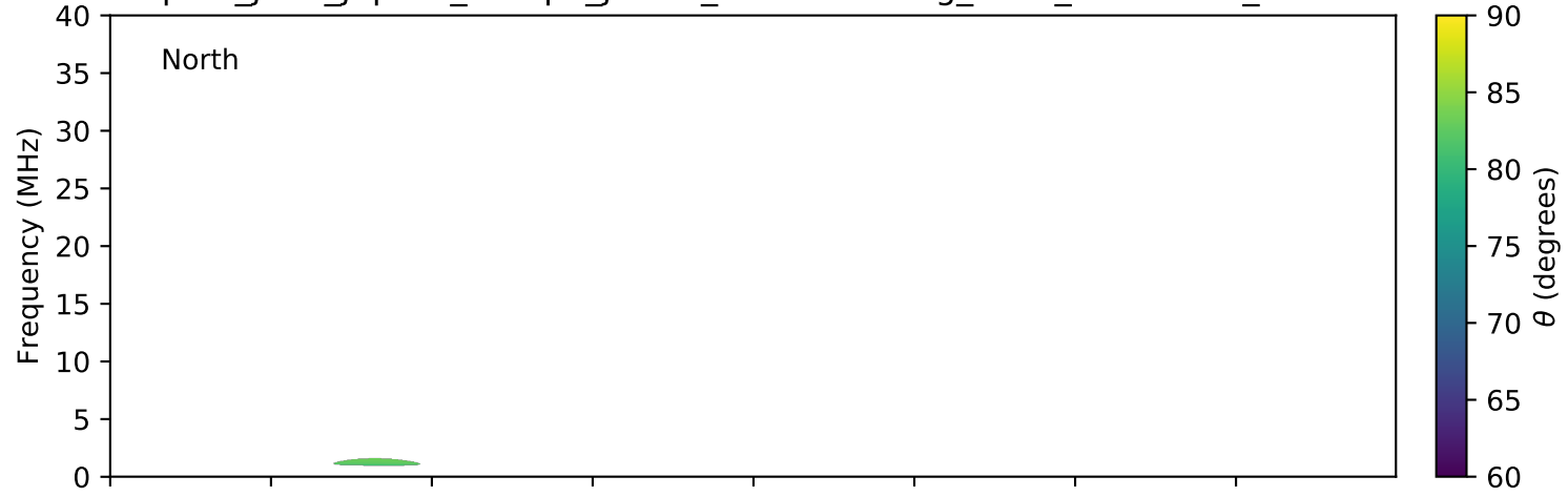
expres_juno_jupiter_europa_jrm09_lossc-wid1deg_3kev_20180208_v01.cdf
