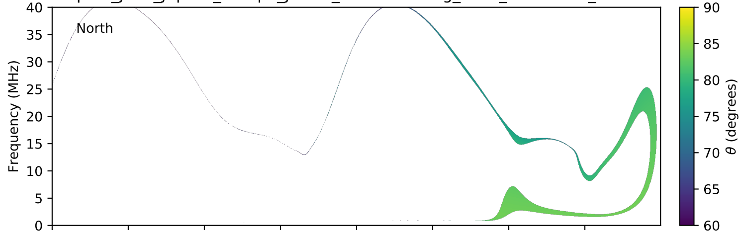
expres_juno_jupiter_europa_jrm09_lossc-wid1deg_3kev_20180206_v01.cdf
