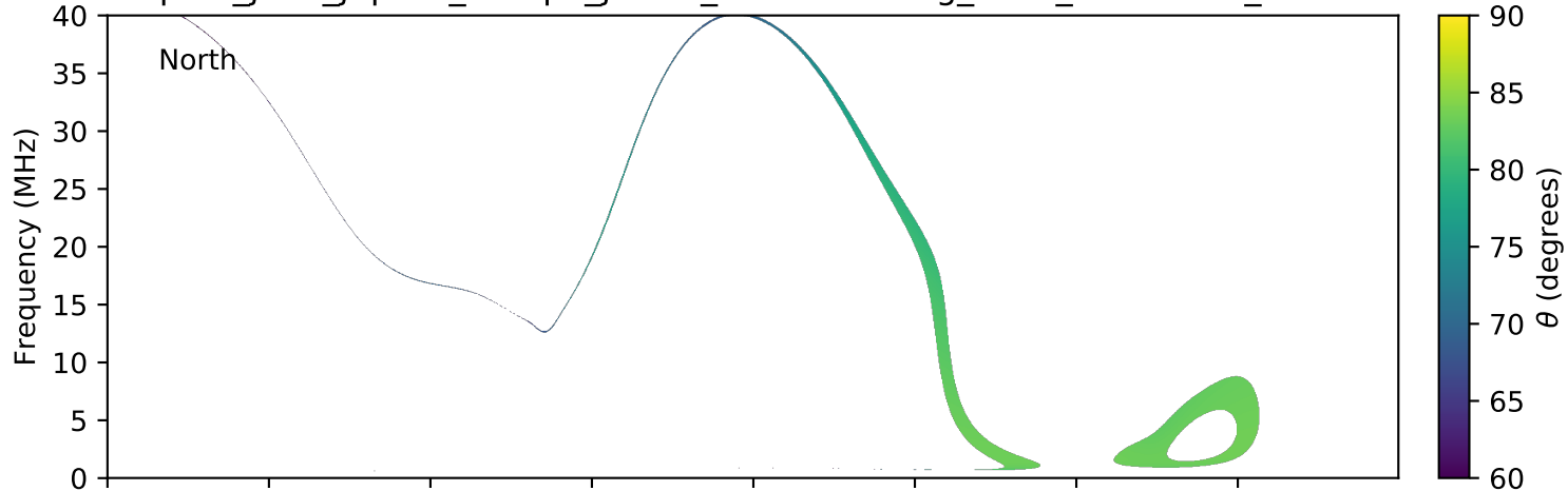
expres_juno_jupiter_europa_jrm09_lossc-wid1deg_3kev_20180204_v01.cdf
