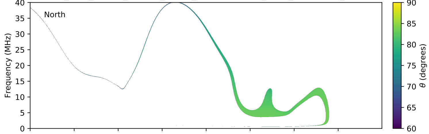
expres_juno_jupiter_europa_jrm09_lossc-wid1deg_3kev_20180202_v01.cdf
