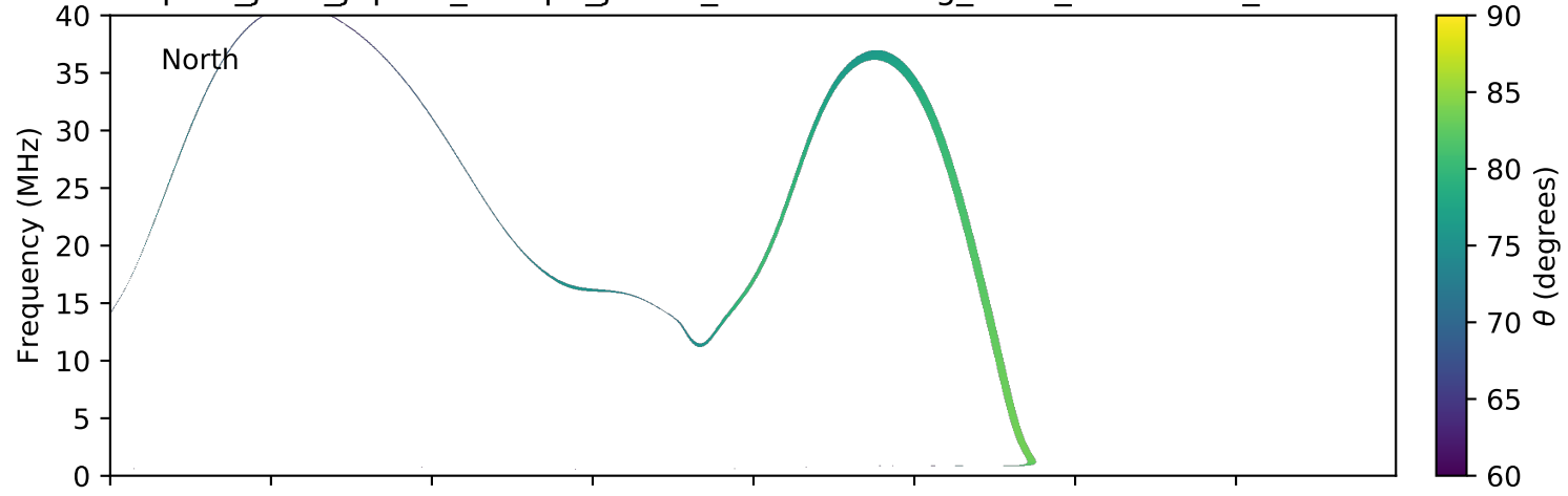
expres_juno_jupiter_europa_jrm09_lossc-wid1deg_3kev_20180201_v01.cdf
