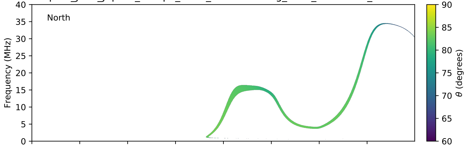
expres_juno_jupiter_europa_isaac_lossc-wid1deg_3kev_20180225_v01.cdf
