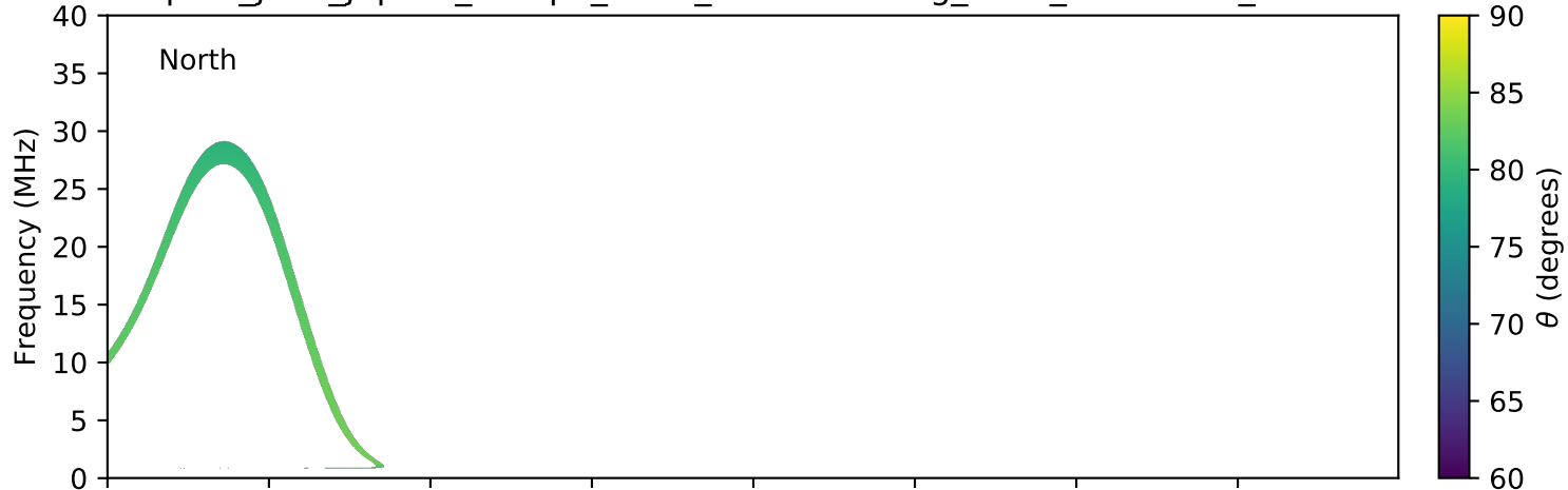
expres_juno_jupiter_europa_isaac_lossc-wid1deg_3kev_20180223_v01.cdf
