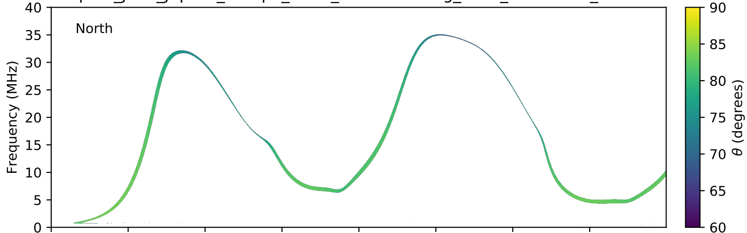
expres_juno_jupiter_europa_isaac_lossc-wid1deg_3kev_20180222_v01.cdf
