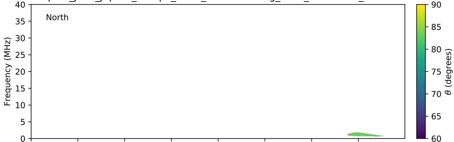
expres_juno_jupiter_europa_isaac_lossc-wid1deg_3kev_20180221_v01.cdf
