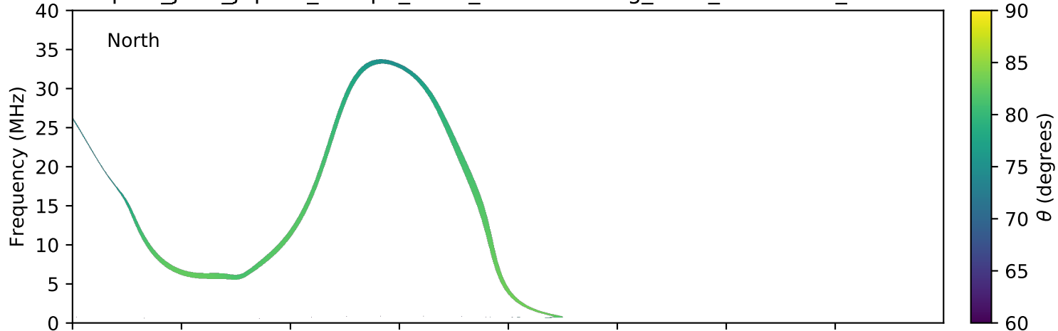
expres_juno_jupiter_europa_isaac_lossc-wid1deg_3kev_20180219_v01.cdf
