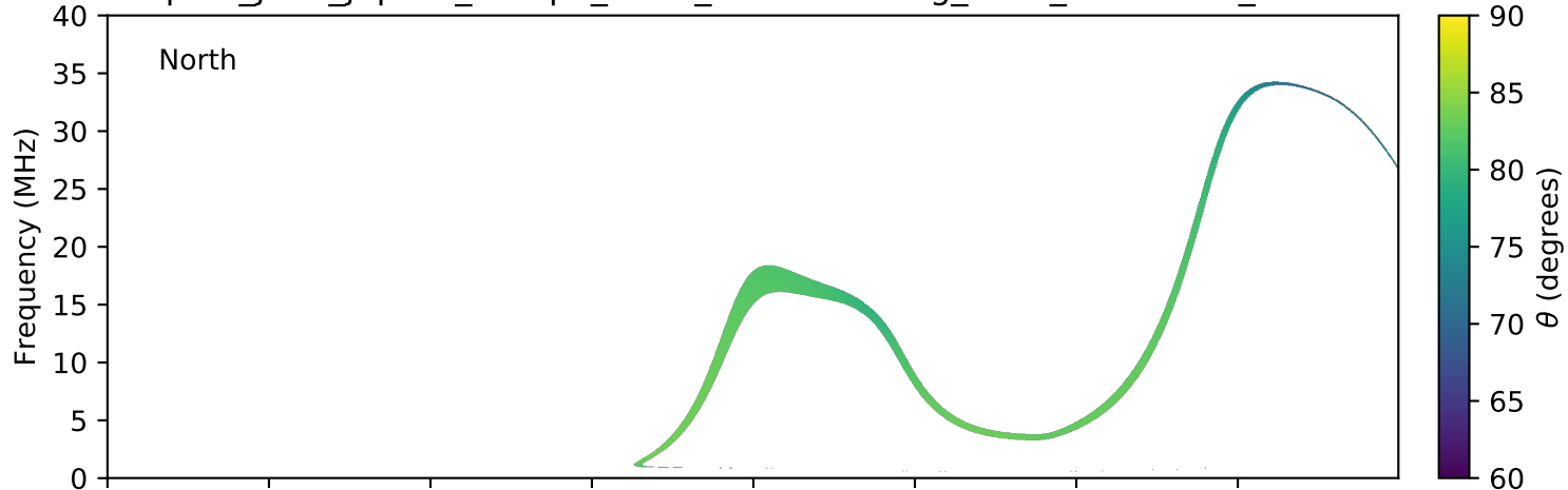
expres_juno_jupiter_europa_isaac_lossc-wid1deg_3kev_20180218_v01.cdf
