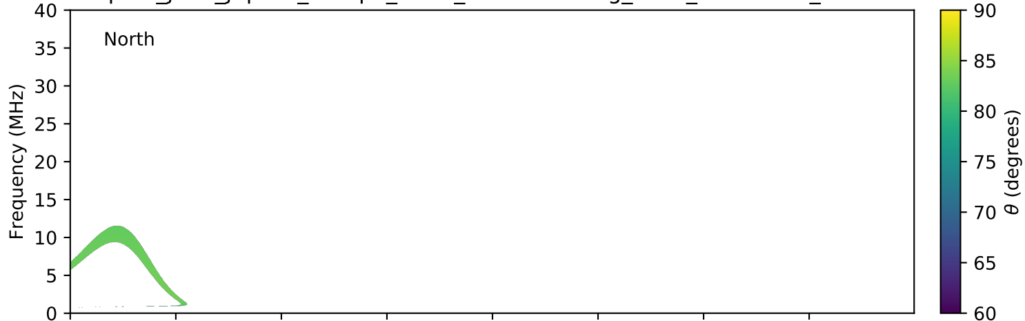
expres_juno_jupiter_europa_isaac_lossc-wid1deg_3kev_20180216_v01.cdf
