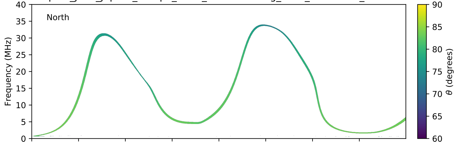
expres_juno_jupiter_europa_isaac_lossc-wid1deg_3kev_20180215_v01.cdf
