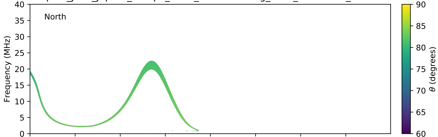
expres_juno_jupiter_europa_isaac_lossc-wid1deg_3kev_20180212_v01.cdf
