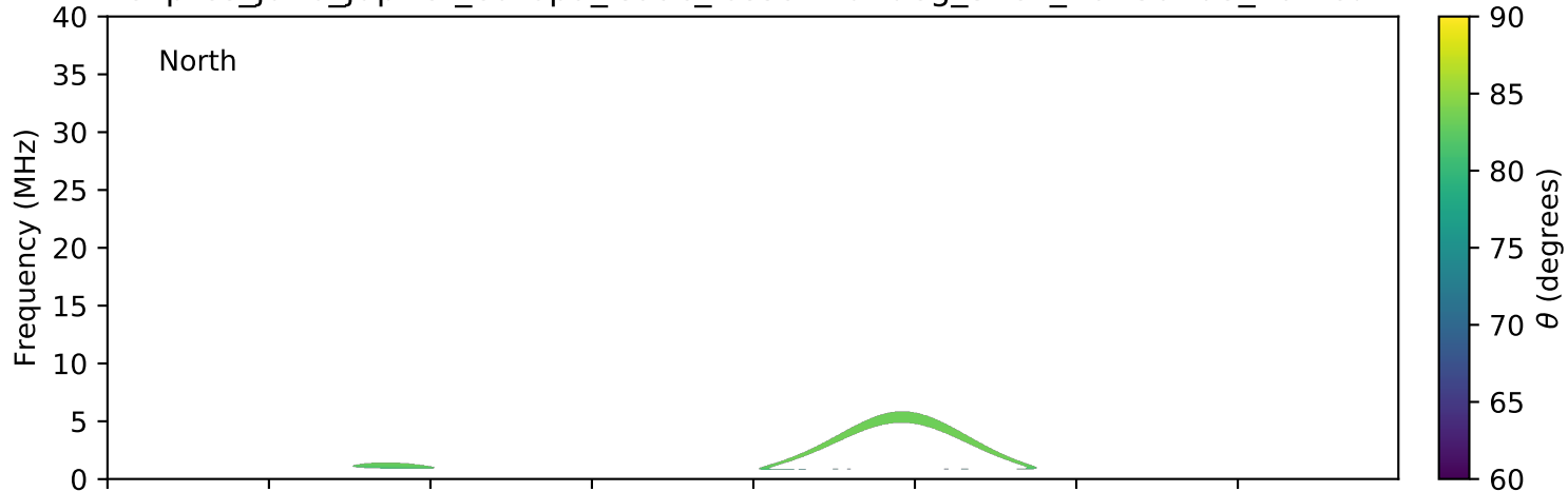
expres_juno_jupiter_europa_isaac_lossc-wid1deg_3kev_20180208_v01.cdf
