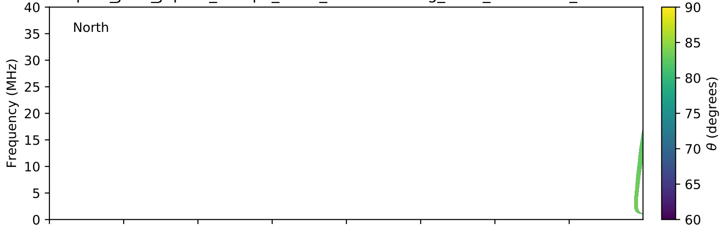
expres_juno_jupiter_europa_isaac_lossc-wid1deg_3kev_20180203_v01.cdf
