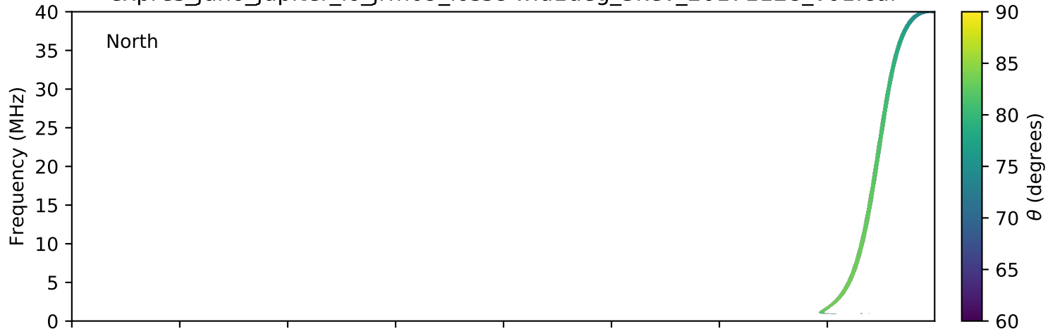
expres_juno_jupiter_io_jrm09_lossc-wid1deg_3kev_20171128_v01.cdf
