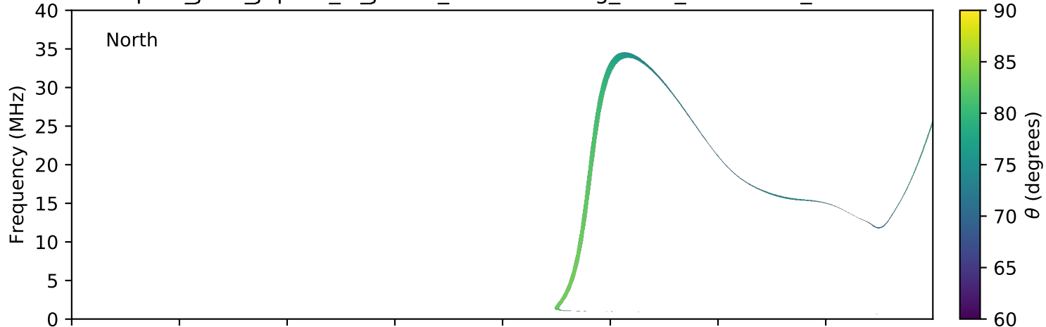
expres_juno_jupiter_io_jrm09_lossc-wid1deg_3kev_20171123_v01.cdf
