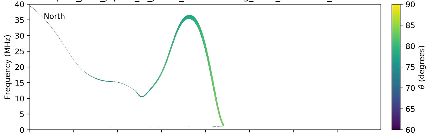
expres_juno_jupiter_io_jrm09_lossc-wid1deg_3kev_20171122_v01.cdf
