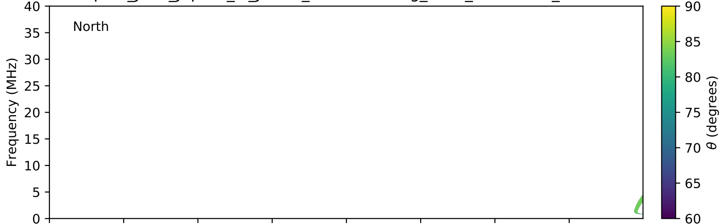
expres_juno_jupiter_io_jrm09_lossc-wid1deg_3kev_20171119_v01.cdf
