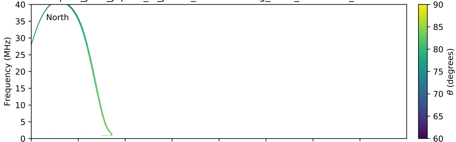
expres_juno_jupiter_io_jrm09_lossc-wid1deg_3kev_20171117_v01.cdf
