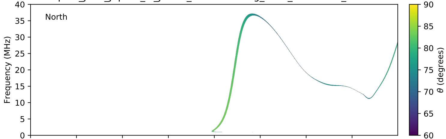
expres_juno_jupiter_io_jrm09_lossc-wid1deg_3kev_20171116_v01.cdf
