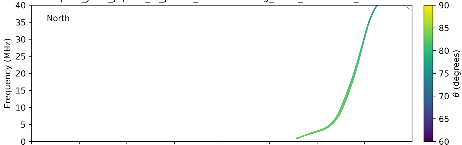
expres_juno_jupiter_io_jrm09_lossc-wid1deg_3kev_20171114_v01.cdf
