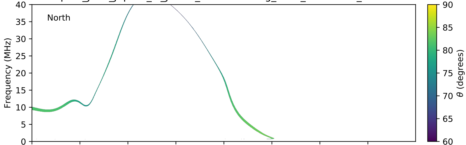
expres_juno_jupiter_io_jrm09_lossc-wid1deg_3kev_20171113_v01.cdf
