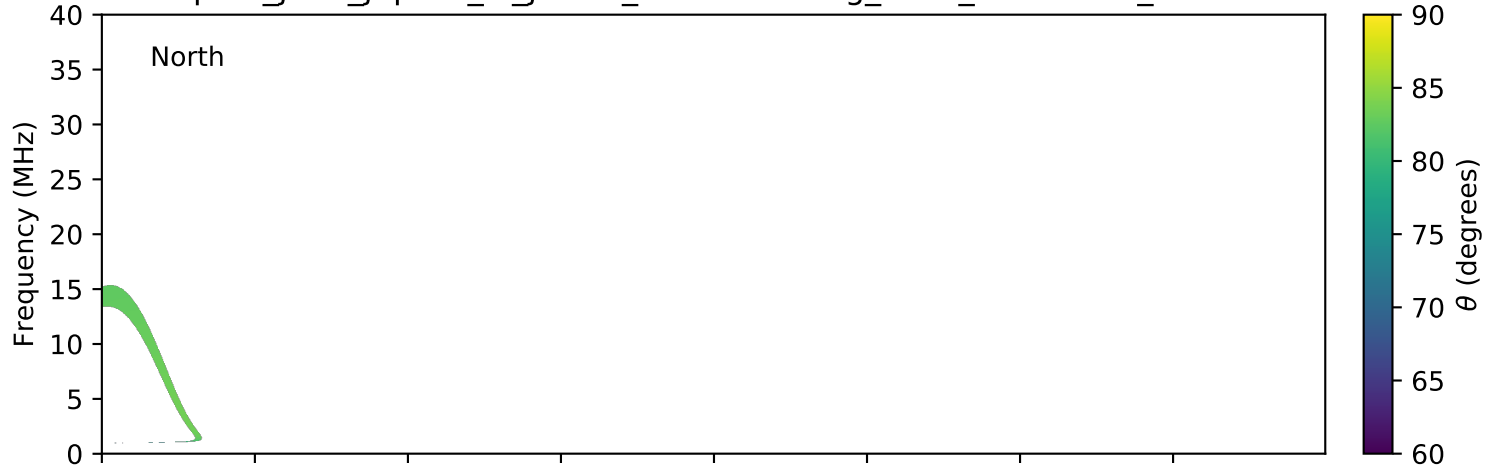
expres_juno_jupiter_io_jrm09_lossc-wid1deg_3kev_20171103_v01.cdf
