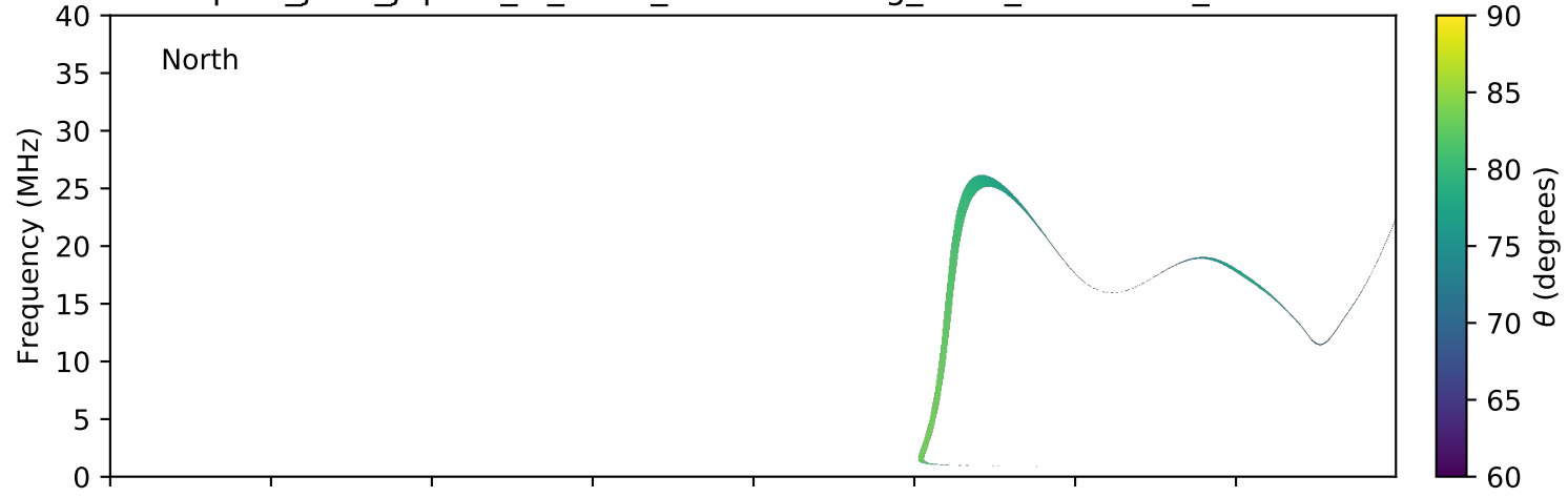
expres_juno_jupiter_io_isaac_lossc-wid1deg_3kev_20171130_v01.cdf
