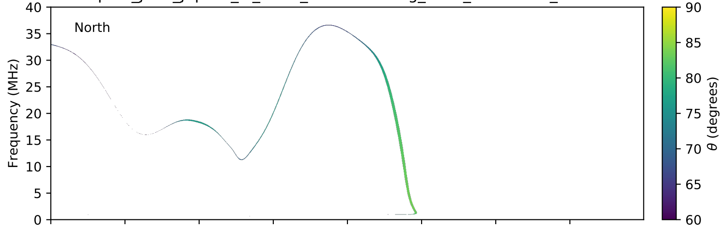
expres_juno_jupiter_io_isaac_lossc-wid1deg_3kev_20171129_v01.cdf
