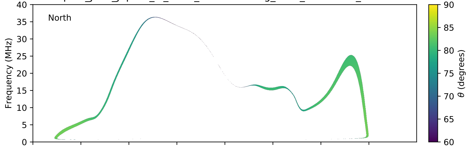
expres_juno_jupiter_io_isaac_lossc-wid1deg_3kev_20171127_v01.cdf
