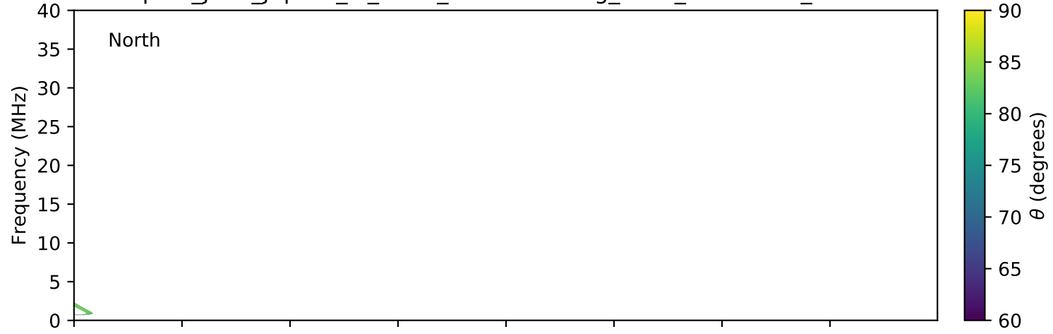
expres_juno_jupiter_io_isaac_lossc-wid1deg_3kev_20171126_v01.cdf
