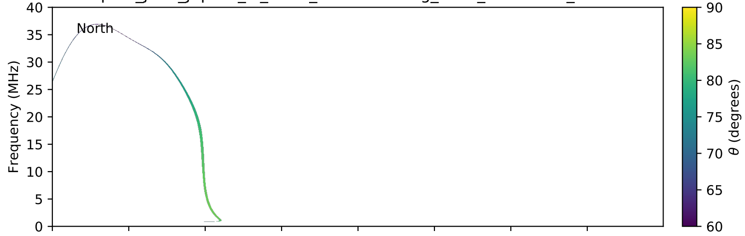
expres_juno_jupiter_io_isaac_lossc-wid1deg_3kev_20171124_v01.cdf
