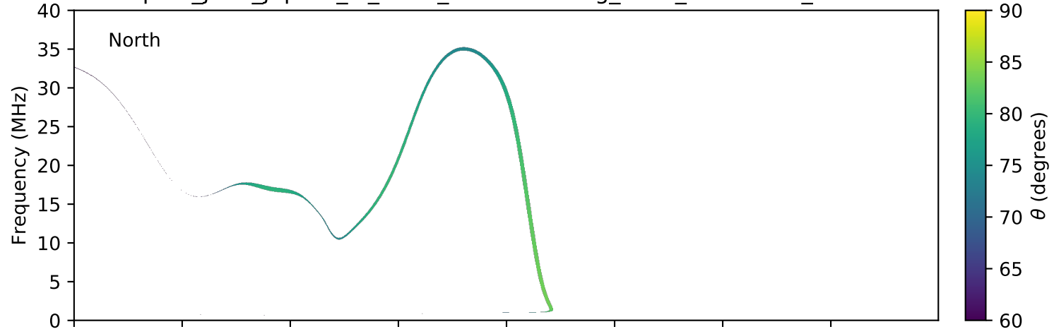
expres_juno_jupiter_io_isaac_lossc-wid1deg_3kev_20171122_v01.cdf
