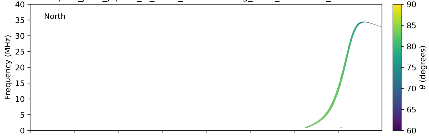
expres_juno_jupiter_io_isaac_lossc-wid1deg_3kev_20171121_v01.cdf
