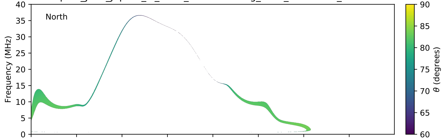
expres_juno_jupiter_io_isaac_lossc-wid1deg_3kev_20171120_v01.cdf
