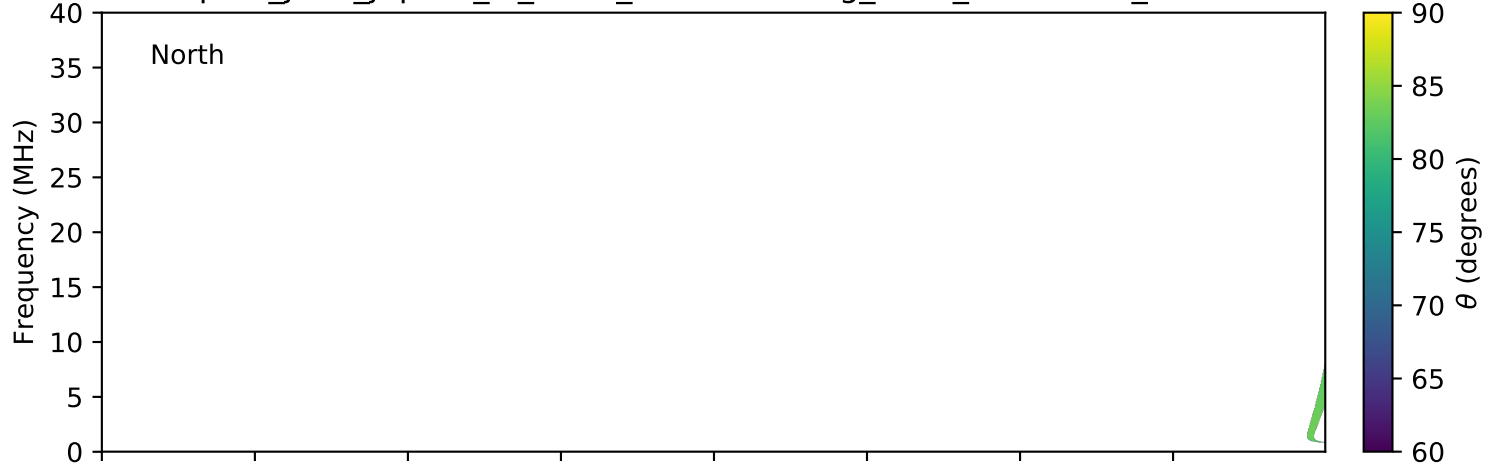
expres_juno_jupiter_io_isaac_lossc-wid1deg_3kev_20171119_v01.cdf
