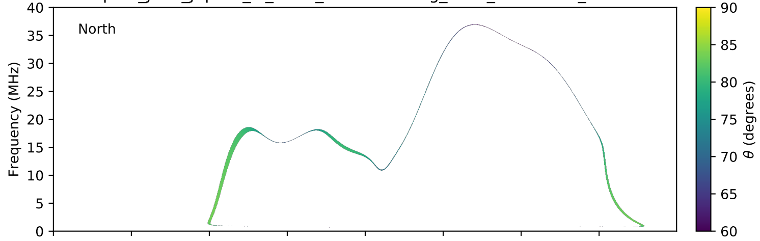
expres_juno_jupiter_io_isaac_lossc-wid1deg_3kev_20171118_v01.cdf
