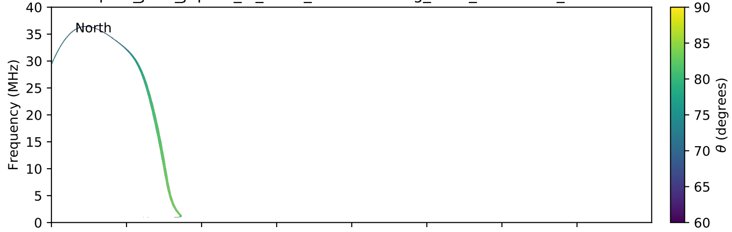
expres_juno_jupiter_io_isaac_lossc-wid1deg_3kev_20171117_v01.cdf
