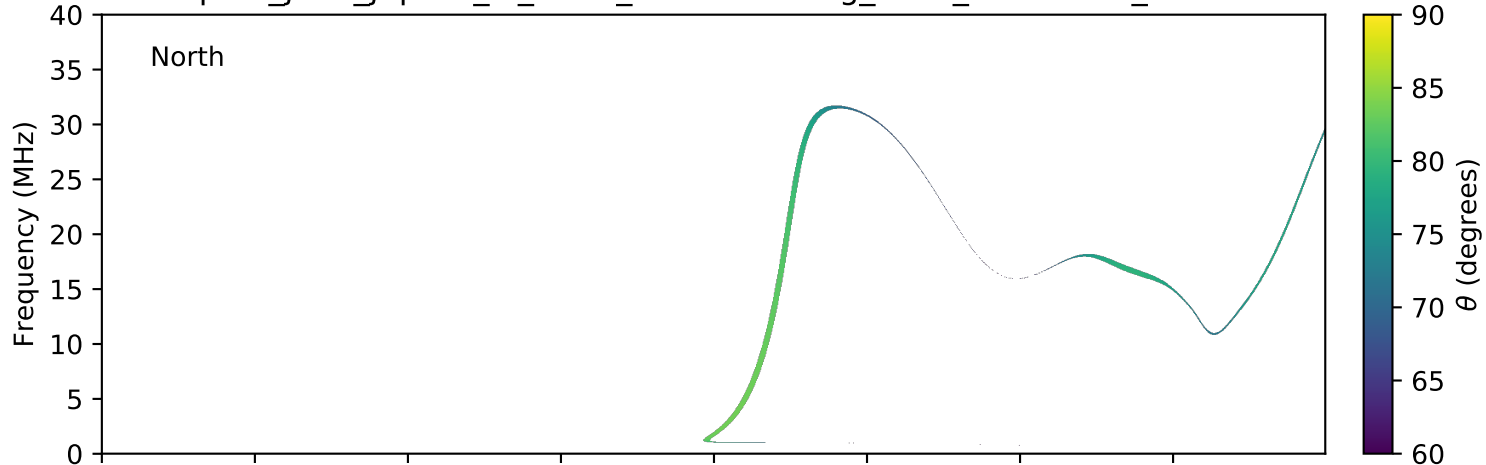
expres_juno_jupiter_io_isaac_lossc-wid1deg_3kev_20171116_v01.cdf
