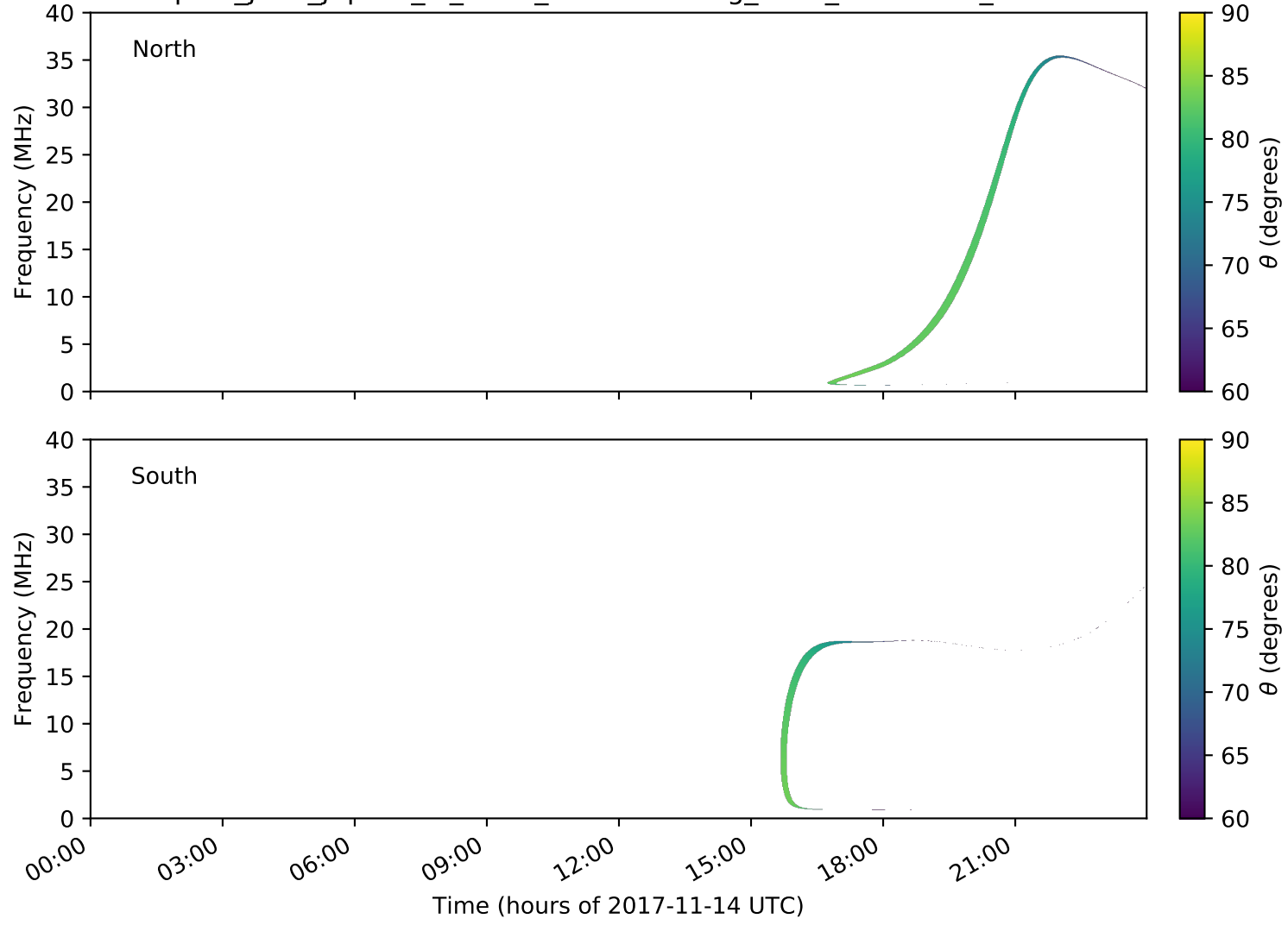
expres_juno_jupiter_io_isaac_lossc-wid1deg_3kev_20171114_v01.cdf
