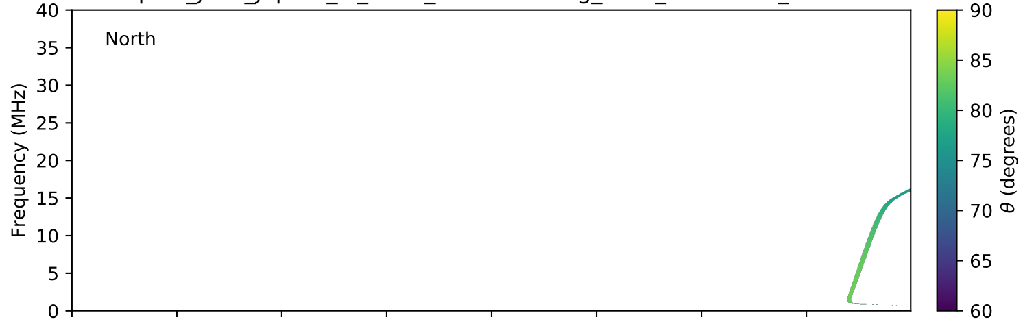
expres_juno_jupiter_io_isaac_lossc-wid1deg_3kev_20171112_v01.cdf
