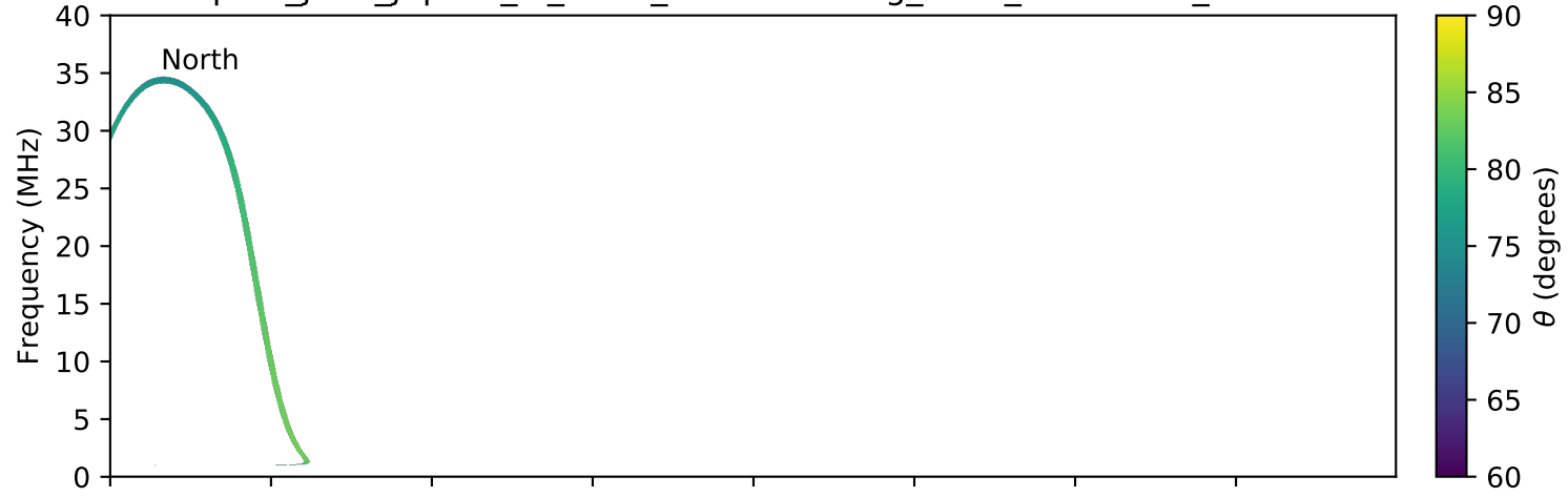
expres_juno_jupiter_io_isaac_lossc-wid1deg_3kev_20171110_v01.cdf
