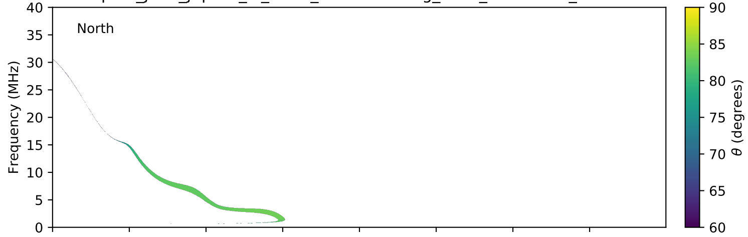
expres_juno_jupiter_io_isaac_lossc-wid1deg_3kev_20171108_v01.cdf
