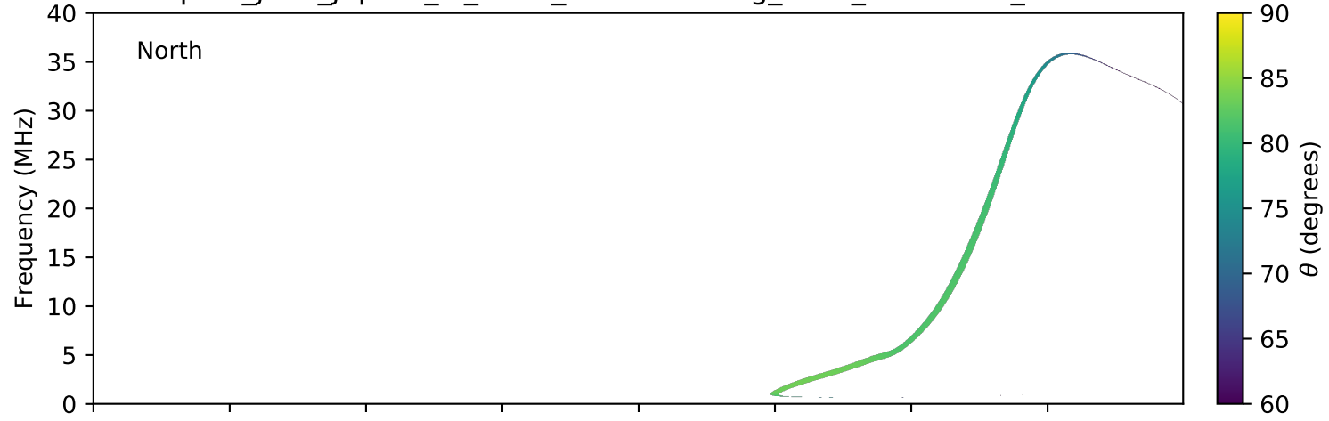
expres_juno_jupiter_io_isaac_lossc-wid1deg_3kev_20171107_v01.cdf
