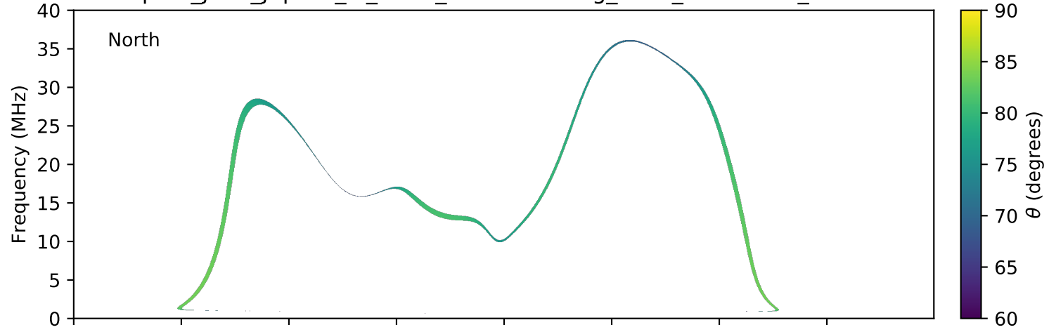
expres_juno_jupiter_io_isaac_lossc-wid1deg_3kev_20171104_v01.cdf
