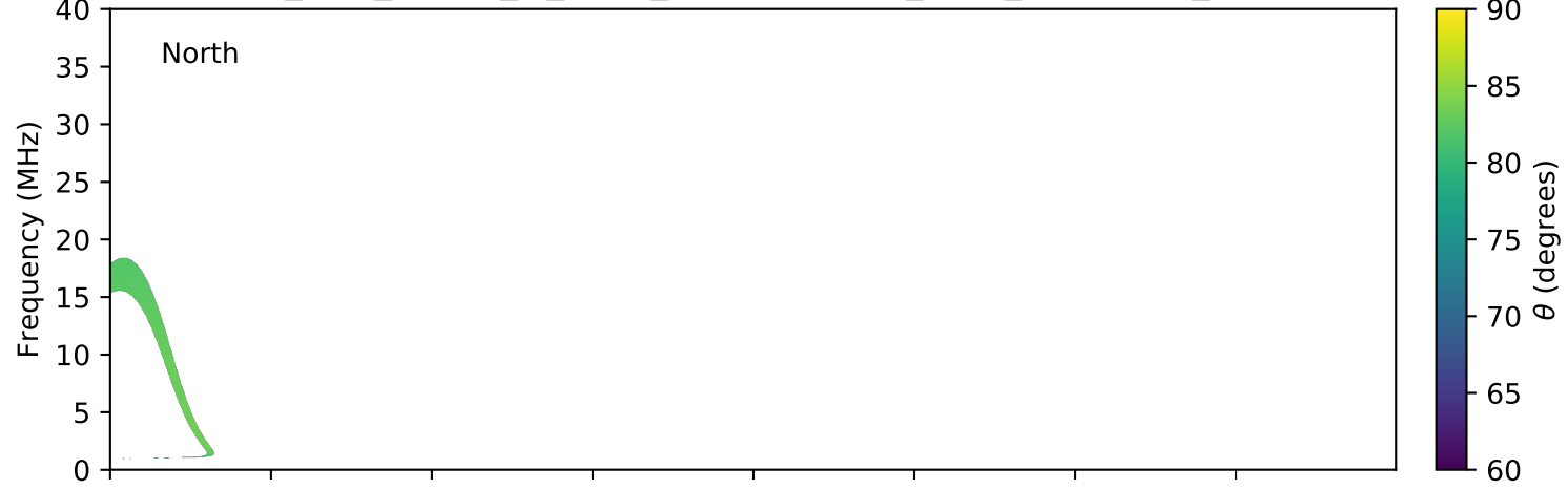
expres_juno_jupiter_io_isaac_lossc-wid1deg_3kev_20171103_v01.cdf
