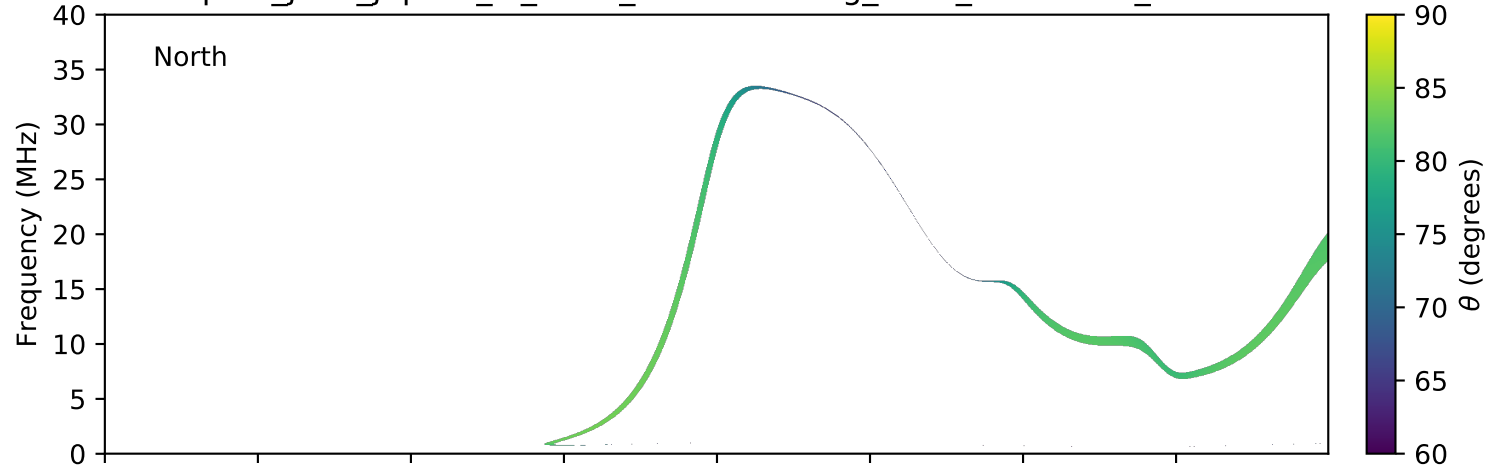
expres_juno_jupiter_io_isaac_lossc-wid1deg_3kev_20171102_v01.cdf
