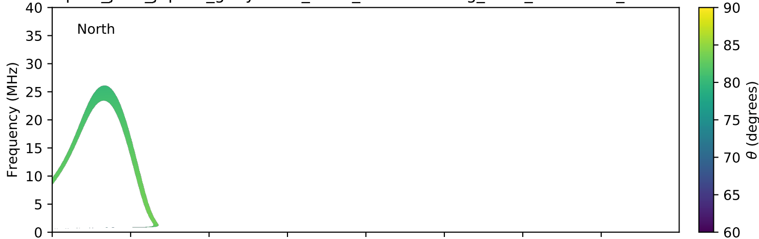
expres_juno_jupiter_ganymede_isaac_lossc-wid1deg_3kev_20171129_v01.cdf
